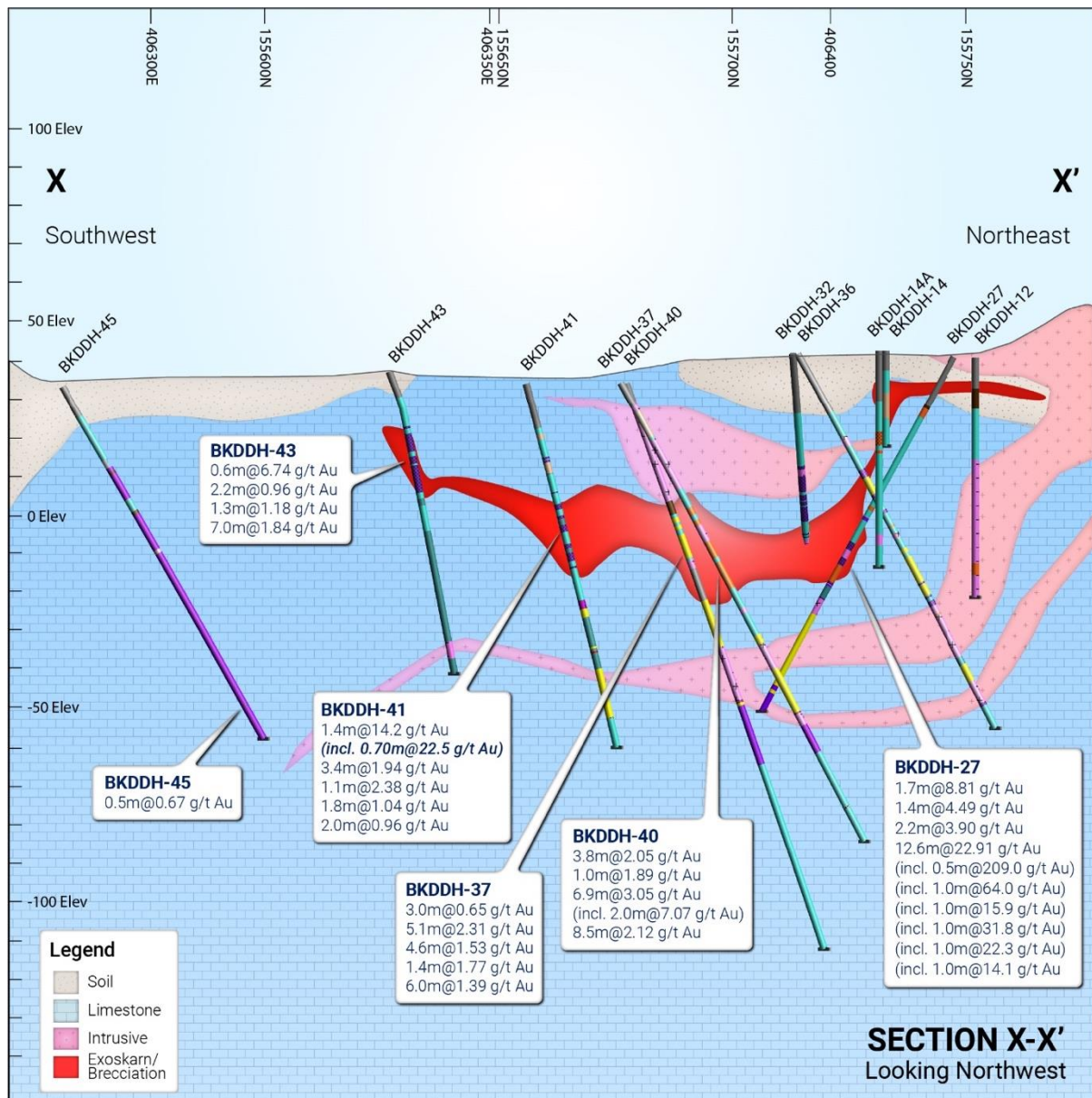
Figure 3: Summary of significant intercepts, highlighting the correlation of the discovery interval in BKDDH-27 with assay results from the follow-up round holes (red interval) projected onto cross-section XX'.
