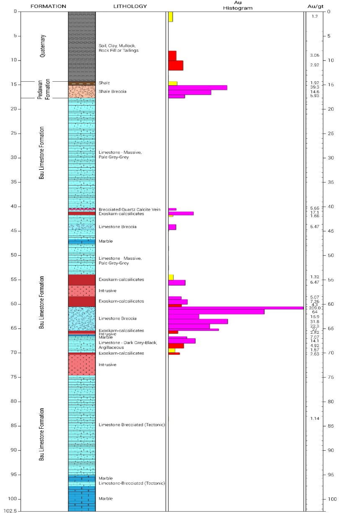
Figure 2: Summary of core lithology and gold assay results for BKDDH-27 showing exceptional gold tenor within two distinct intervals; at the LSC and deeper within the Bau Limestone.
