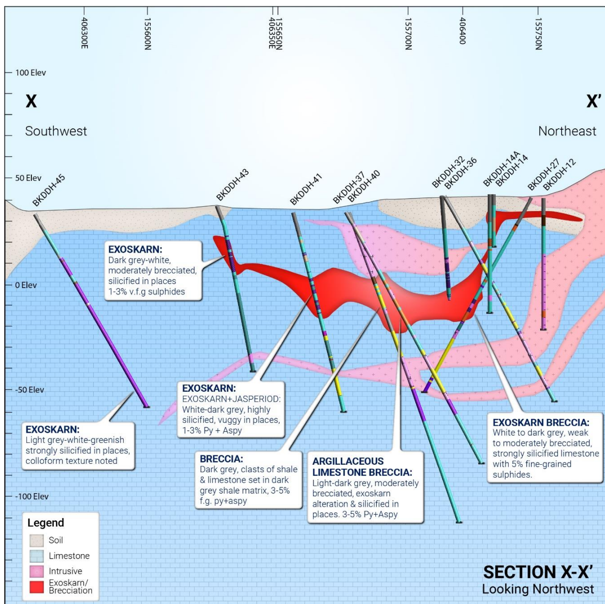
Figure 4: Summary of hydrothermal alteration textures used to provide a signature marker for correlating extensions of the BKDDH-27 discovery interval with intercepts from the follow-up round holes (red interval) projected onto cross-section XX'.
