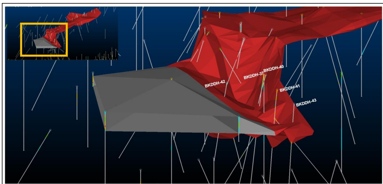
Figure 6: 3D model showing mineralisation (in red) and potential for possible extension (in grey) together with historical drill holes having significant Au intercepts.
